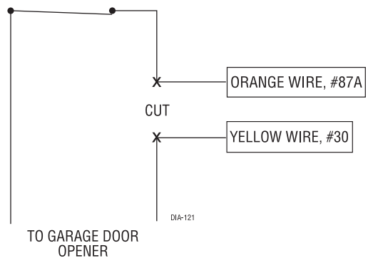
NORMALLY CLOSED SWITCH
