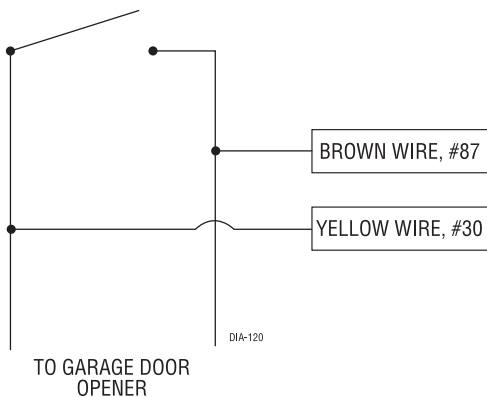
NORMALLY OPEN SWITCH
